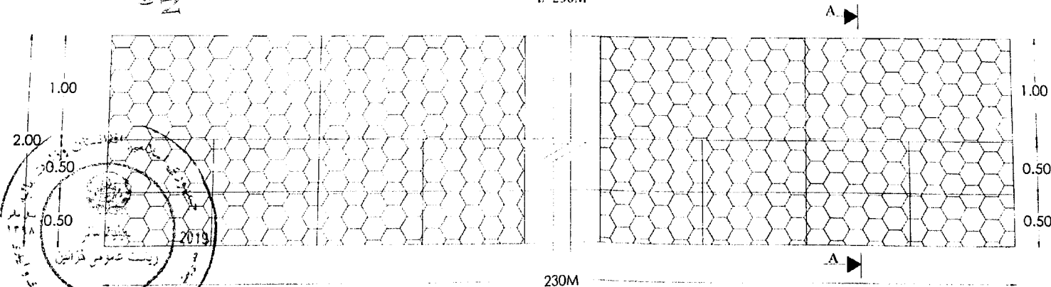
230M Gabion Wall Plan
